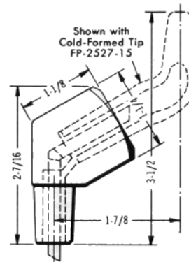
AD-55-30, for 5 RW Tip, Item No. 190-9553
